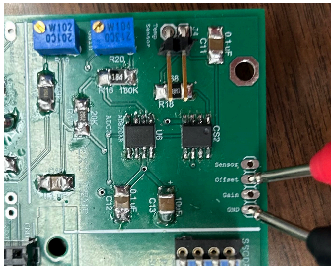
Figure 125: Positioning of multimeter leads to set gain of External Temperature Module.
