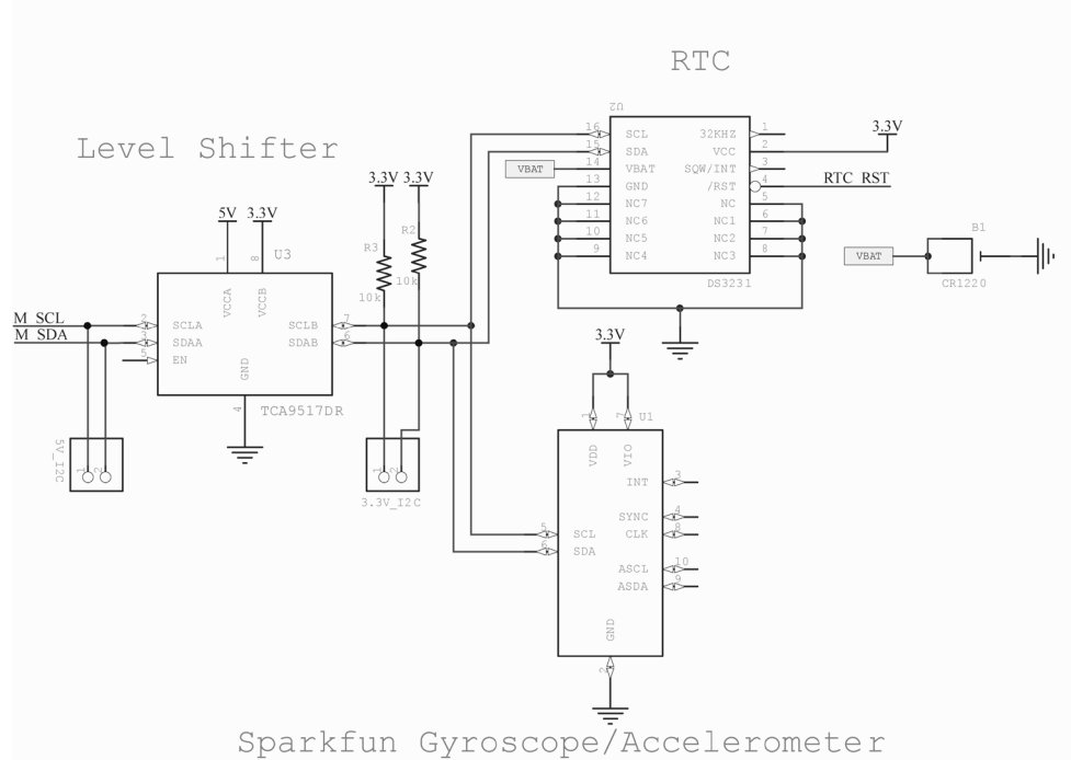
Figure 9: RTC and IMU Module Schematic
