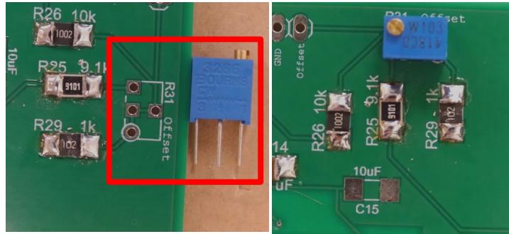
Figure 67: Soldering 10k potentiometer R31.
