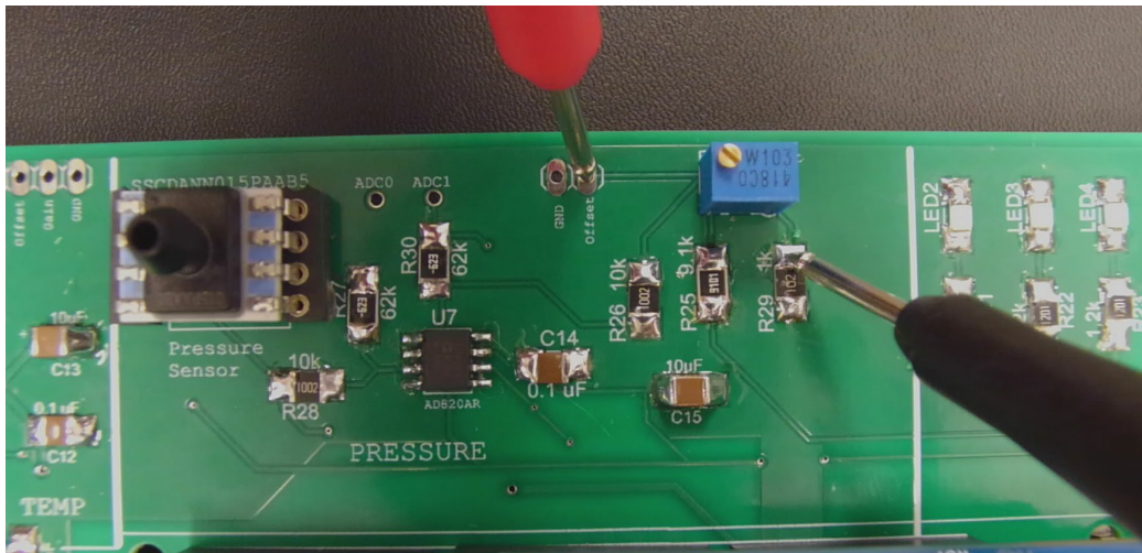
Figure 128: Positioning of the multimeter leads to set and offset of Pressure Module. NOTE THIS IMAGE SHOWS THE PROBE INCORRECTLY ON R29, THE NEGATIVE PROBE SHOULD BE ONE R25 DIRECTLY TO THE LEFT
