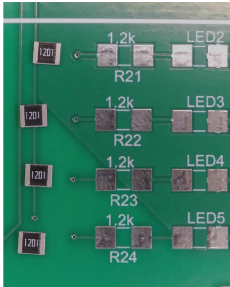
Figure 26: LED Resistors R21, R22, R23, R24.
