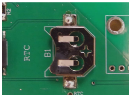
Figure 14: Completely soldered battery holder.
