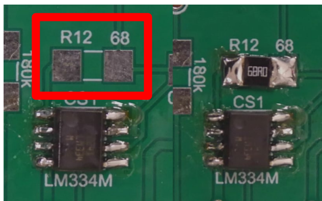
Figure 33: Soldering Resistor R12.
