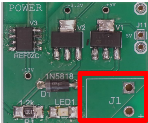
Figure 20: Where jumper J1 will be soldered to the PCB
