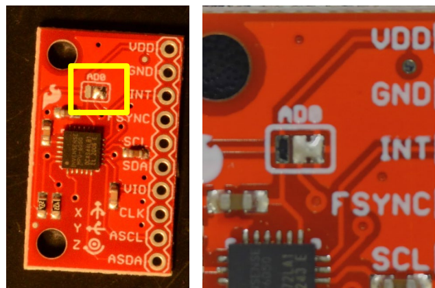
Figure 18: The AD0 jumper on the breakout board. The center pad is connected to an address select pin on the IMU chip. The right pad is connected to ground and the left to VDD (voltage supply). In the shown configuration this sets the address to 0x68
