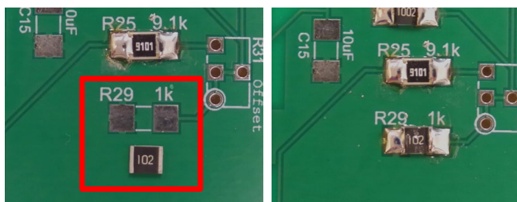
Figure 66: Soldering resistor R29 in place.
