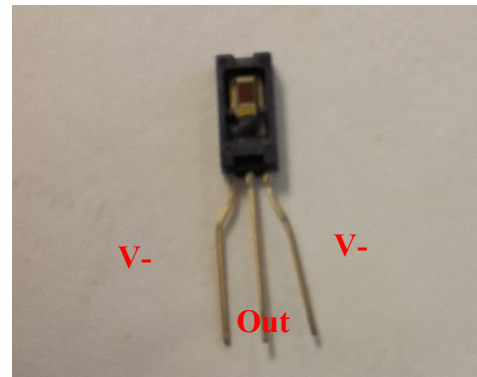
Figure 113: Humidity sensor with pin orientation when viewing sensor.
