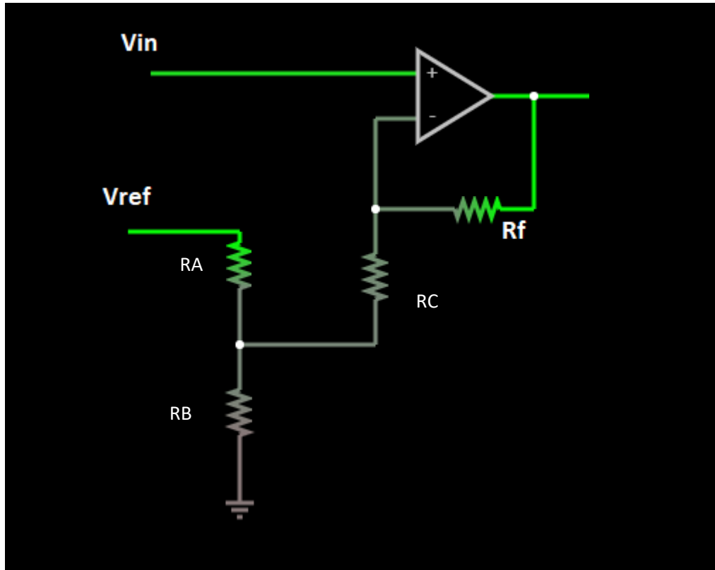
Figure 118: Simplified circuit for Pressure, Temperature and first stage Humidity amplifiers. Not the resistor numbers here are just generic designators and do not correspond to designators on the MegaSat Board. For example, R1 above has nothing to do with R1 on the MegaSat (part of the power circuit). Likewise the values for resistance and voltage should be ignored.
