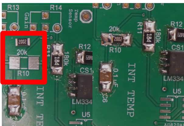
Figure 38: Soldering resistor R10
