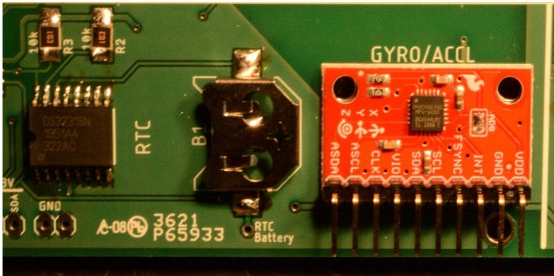
Figure 89: Assembled MPU Module.
