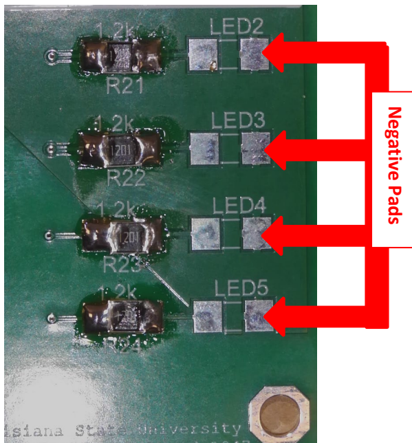
Figure 27 : Negative Pads for LED2, LED3, LED4, and LED5.
