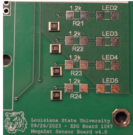
Figure 6: Bare PCB, diagnostic LEDs section
