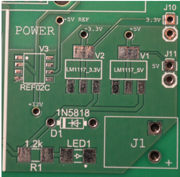
Figure 4: Bare PCB, power distribution section
