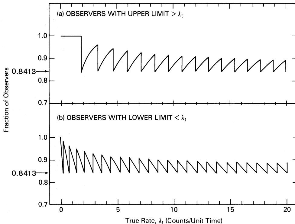
FIG. 2.—Fraction of observers with (a) upper limit greater than the true rate \lambda_t , and (b) lower limit less than \lambda_t , as functions of \lambda_t . For all values of \lambda_t , the fraction is greater than or equal to the confidence level of 0.8413.
