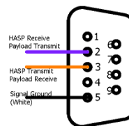
Payload Plate DB-9 connector as viewed from the back of the connector (top of plate)
