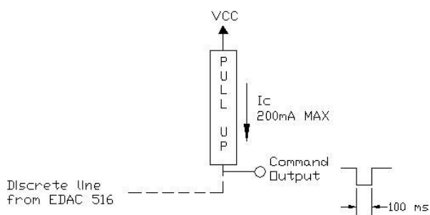
Figure 6: Conditioning circuit for discrete command line interface.
