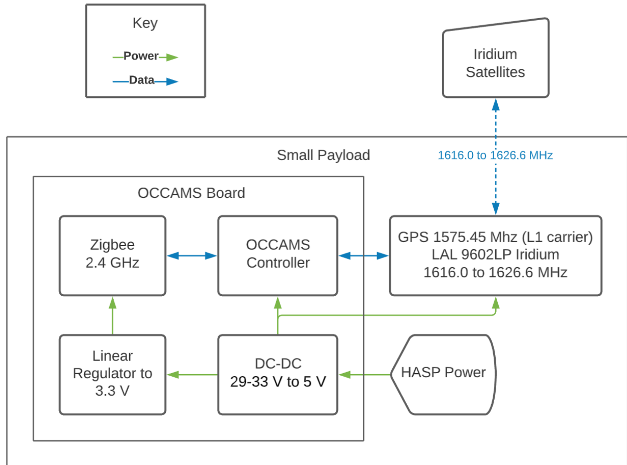
Small Payload Block Diagram
