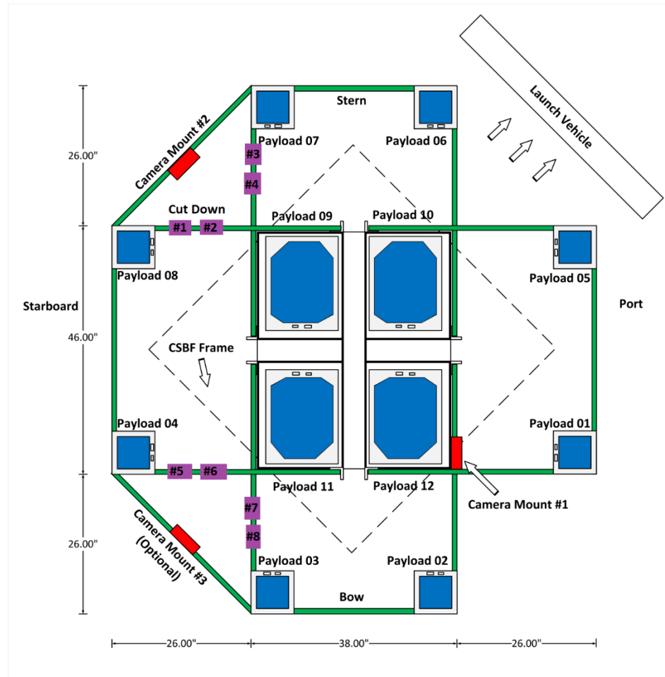
Ideal cut down mounting locations (purple boxes)
