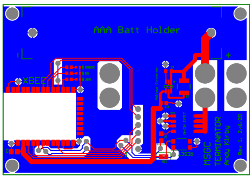
A preliminary board layout for the cutdown board (not containing the redundant, timer-based cutdown mechanism).
