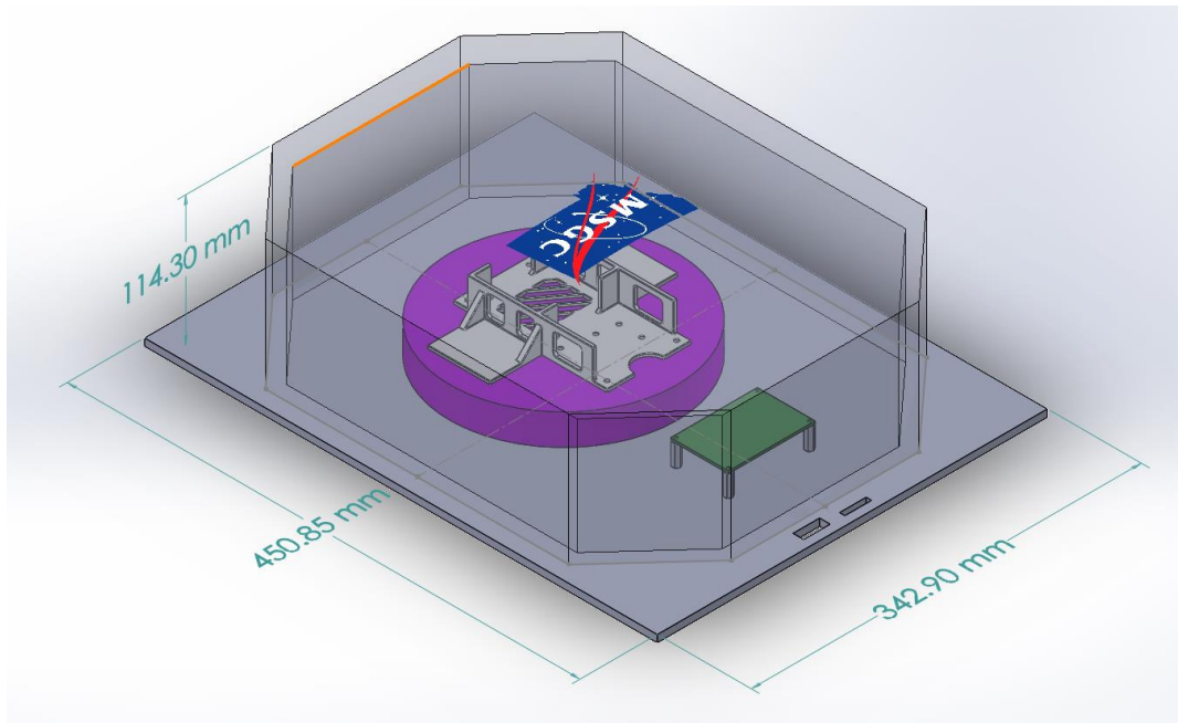
Solidworks model of large payload
