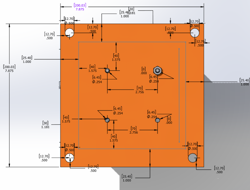
Figure 1: Bottom portion of the Payload attached to plate. Brackets are in millimeters
